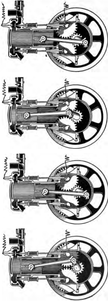
FIG. 127. FIG. 128. FIG. 129. Figs. 127-129. —Sectional Diagrams through a Single Cylinder of a Gasoline Engine, showing the four successive stages in the four-part cycle. In these diagrams both the inlet and exhaust valves are positively operated from cams on secondary shafts. The cam shafts, as shown, being on a two-to-one reduction, turn half as fast as the main shaft. Fig. 127 shows the cams and piston in the position of half way through the inlet stroke, when, as seen, the inlet valve is held open. Fig. 127 shows the beginning of the compression stroke, all valves being closed. Fig. 128 shows the engine ready for firing, all valves still closed. Fig. 129 shows the end of the firing stroke and the beginning of the exhaust, the exhaust valve being open. The view of the engine is that seen when looking toward the front of the vehicle. The fly-wheel rotates clockwise; the cam shafts counter-clockwise.
